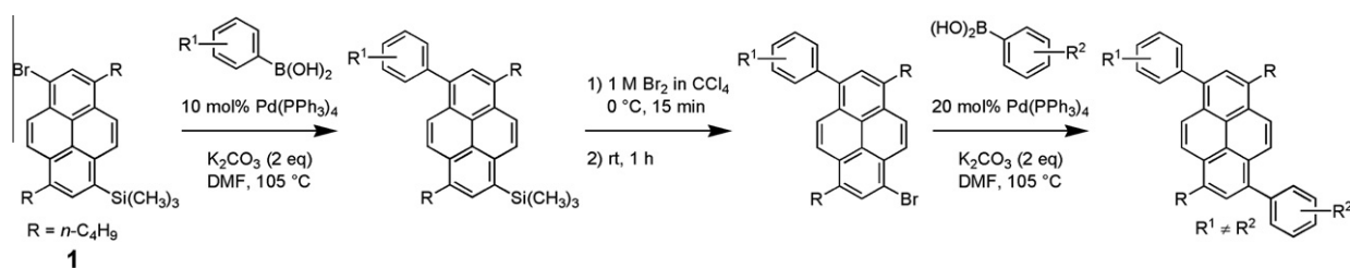
Scheme 1. The outline of synthetic route to unsymmetrically substituted pyrene via 1 .
