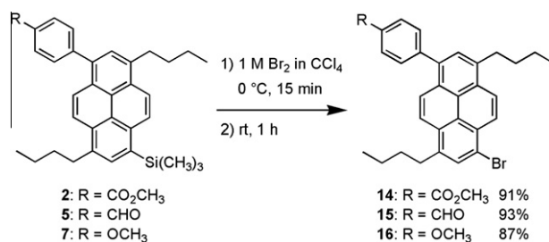
Scheme 3. Desilylation of 2 , 5 , and 7 with bromine.
