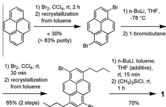
Scheme 2. Synthesis of 1 .
