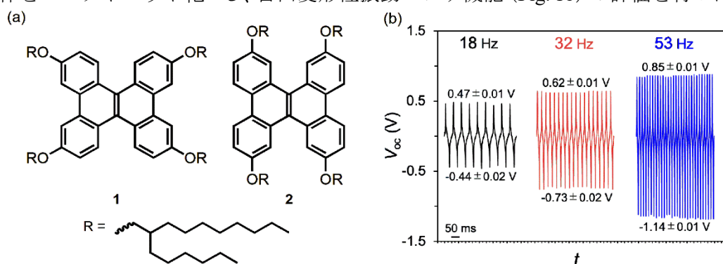
Fig. 1. (a) Molecular structure of alkylated dibenzo[g,p]chrysene liquid derivatives ( 1 , 2 ); (b) Open circuit voltage ( V_{oc} ) characteristics of fabricated mechano-electric generators of the electretized 2 under continuous vibration at different frequencies (18, 32, and 53 Hz).
