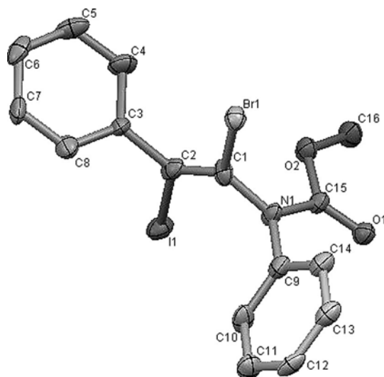
Figure 1. ORTEP drawing of 2 with thermal ellipsoids at the 50% probability level. Hydrogen atoms are omitted for clarity. Selected bond lengths [Å]: N(1)–C(1) = 1.417, C(1)–Br(1) = 1.934, C(2)–I(1) = 2.114, C(1)–C(2) = 1.304.
