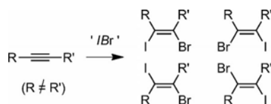
Scheme 1. Iodobromination of alkynes for synthesis of vicinal bromoiodoenamides.
