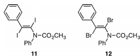
Figure 2. Iodide 11 and bromide 12 .
