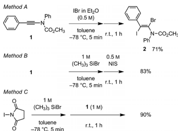
Scheme 2. Regio- and stereoselective iodobromination of 1 to synthesize 2 .
