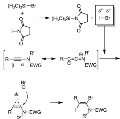
Scheme 3. Plausible reaction mechanism.
